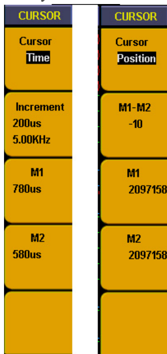
Fig.5-79: Cursor measurement menu
