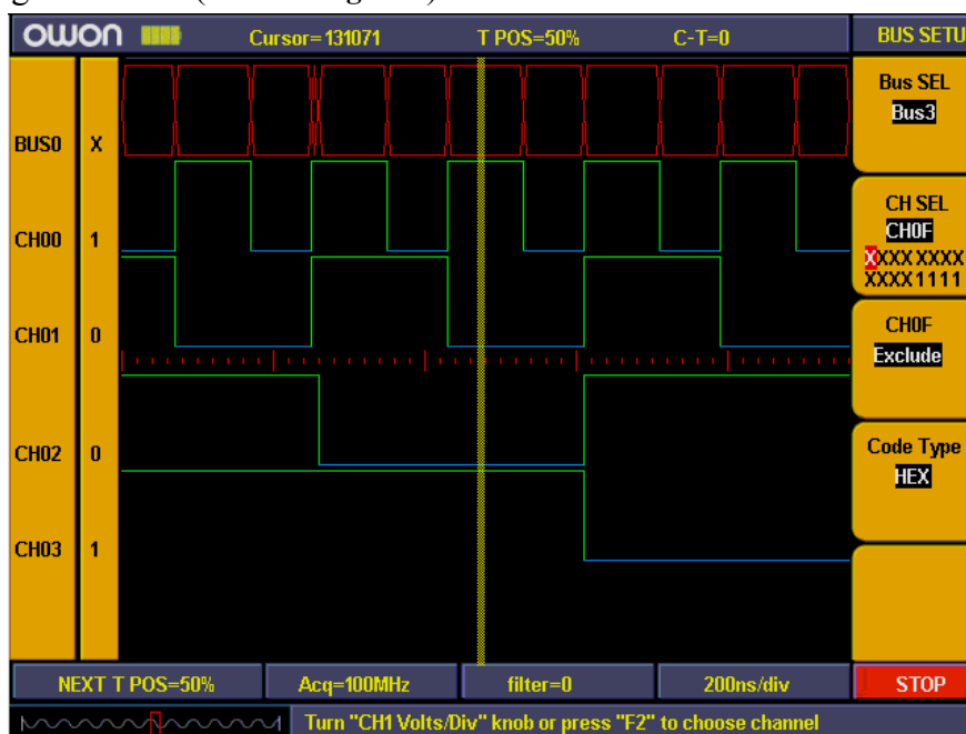
Fig.5-71: Bus setting
