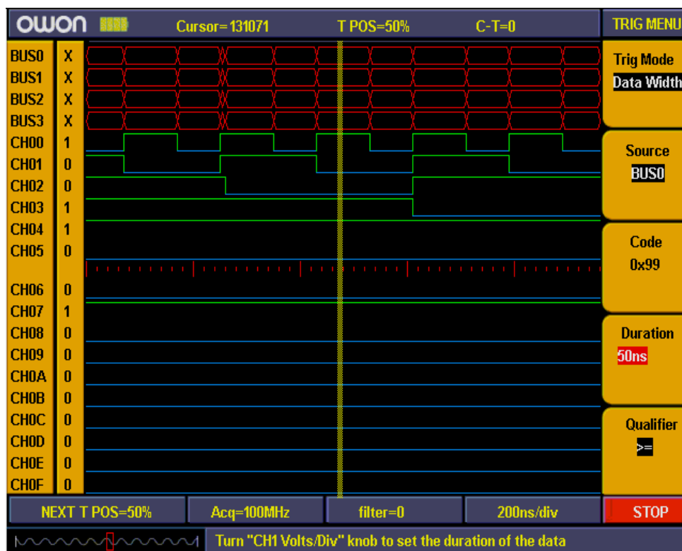
Fig.5-65: Data width trigger
