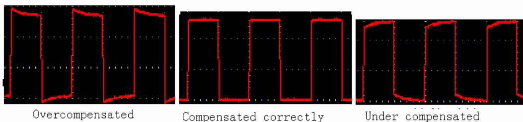
Fig. 4-5 Displayed Wave Forms of the Probe Compensation
