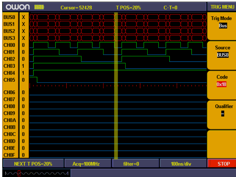
Fig.5-57: Bus trigger
